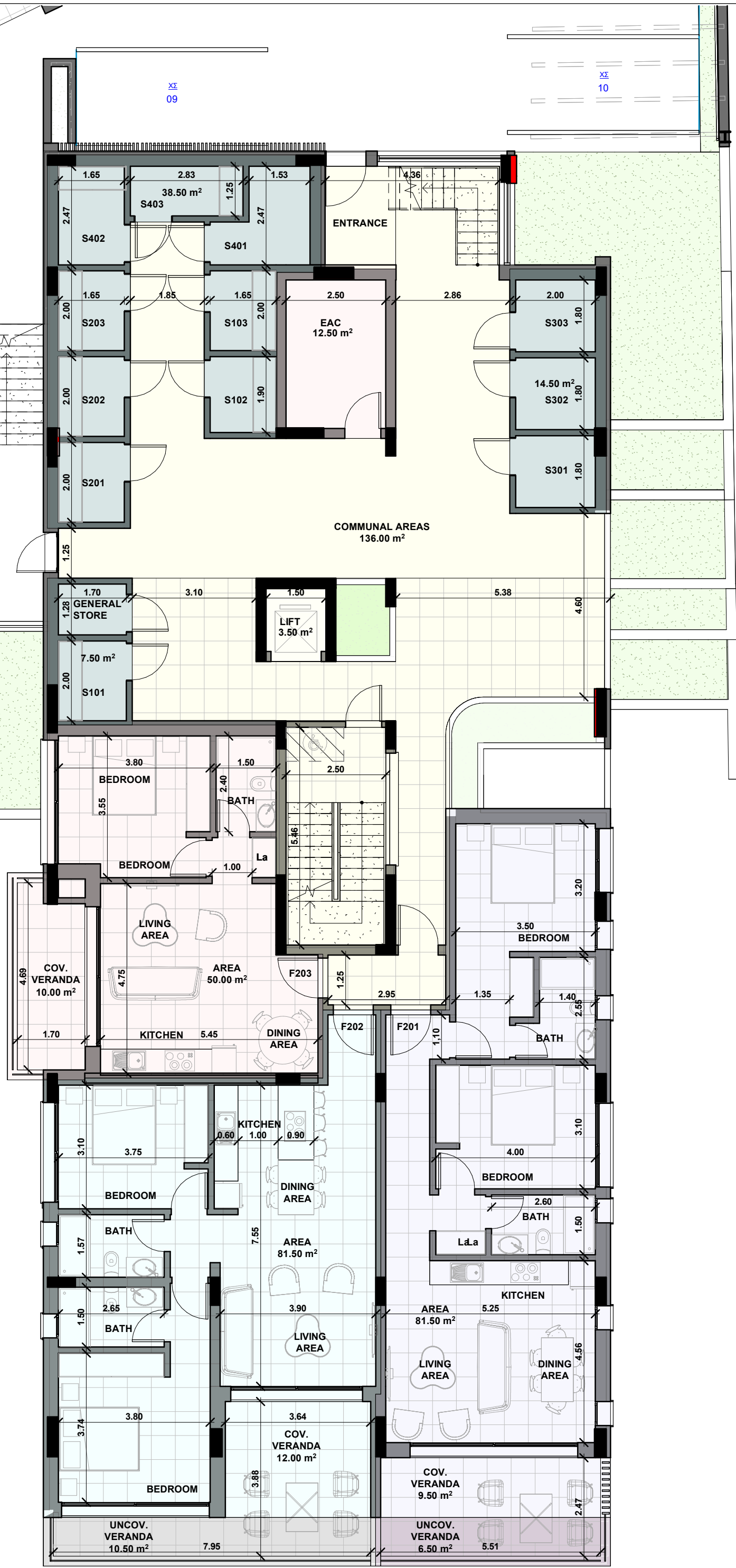
1 • PRES _ LOWER PART _ 2ND LEVEL / UPPER PART _ BASEMENT 1 : 100
