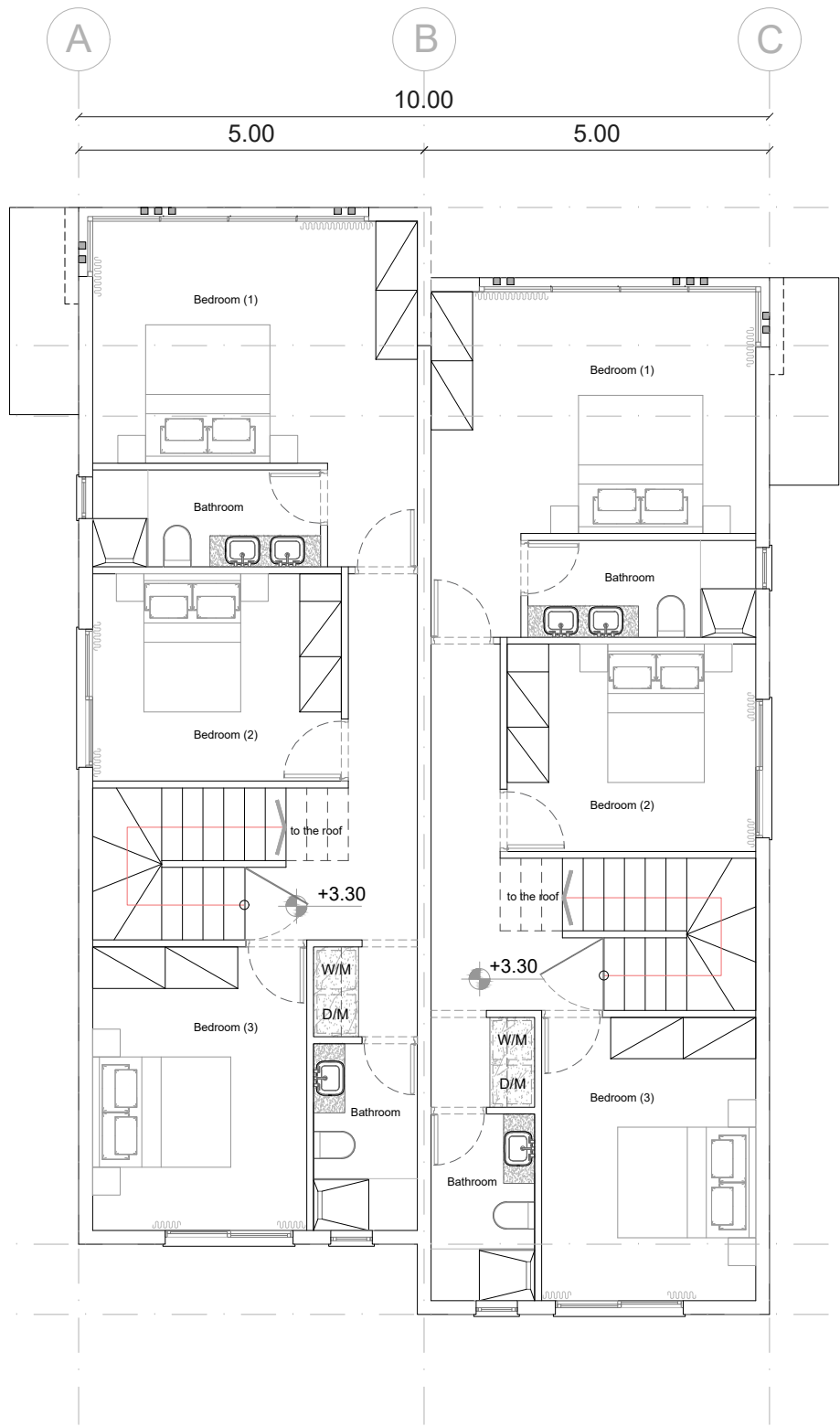
FIRST FLOOR
