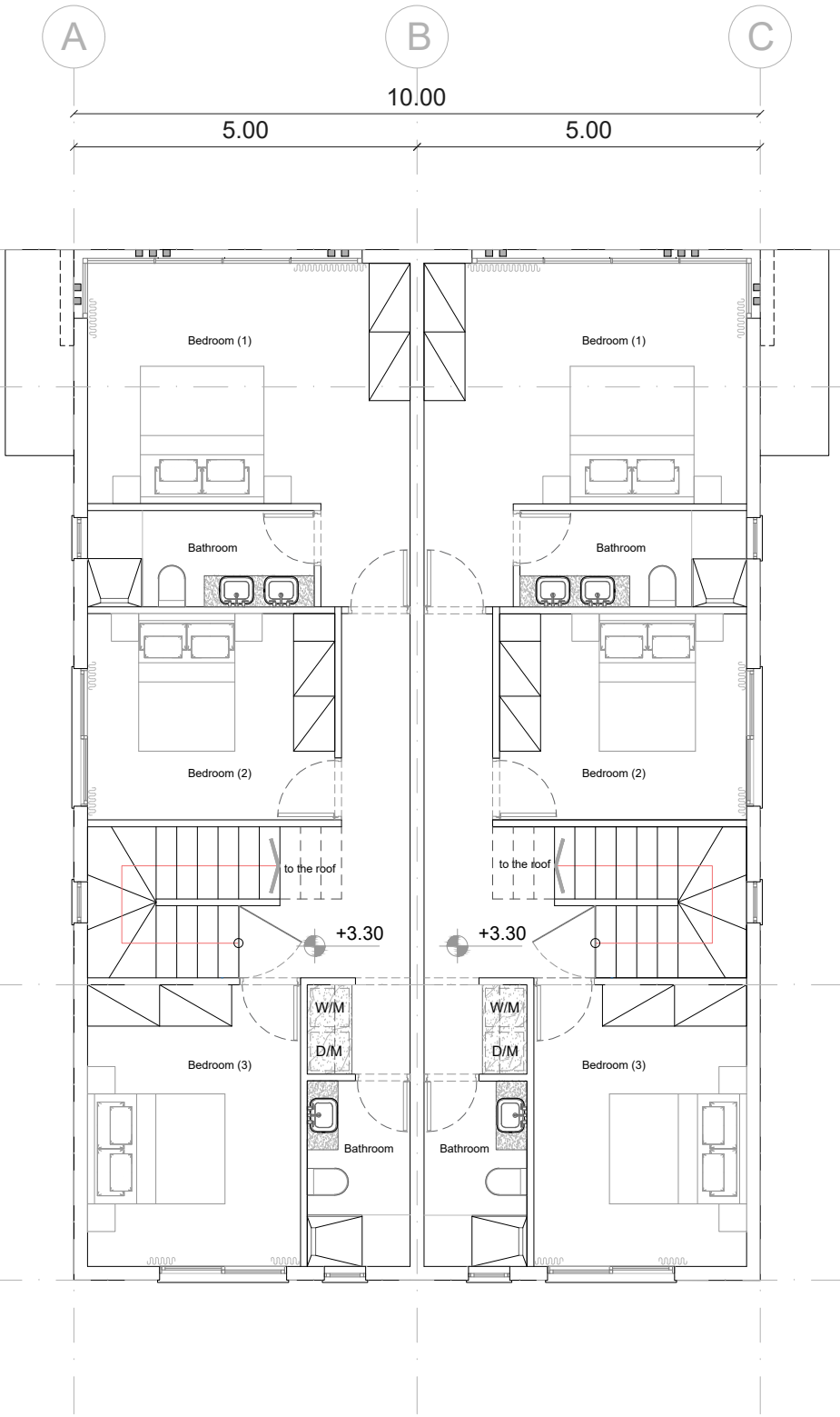
FIRST FLOOR
