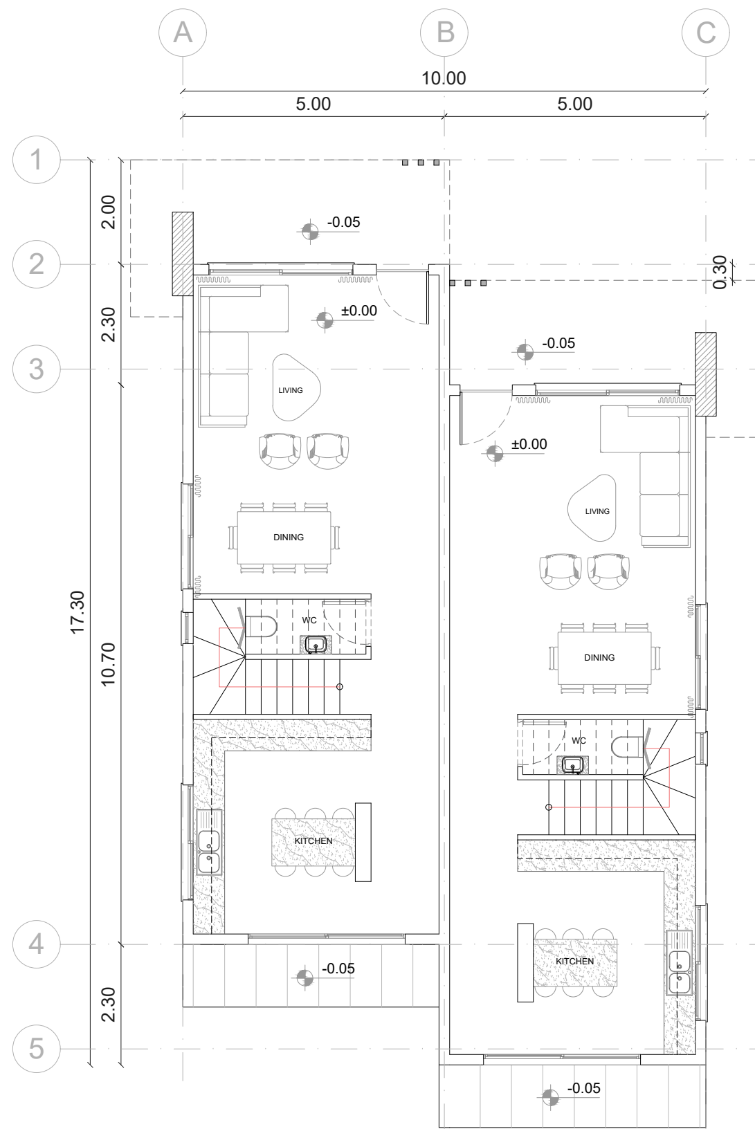
GROUND FLOOR
