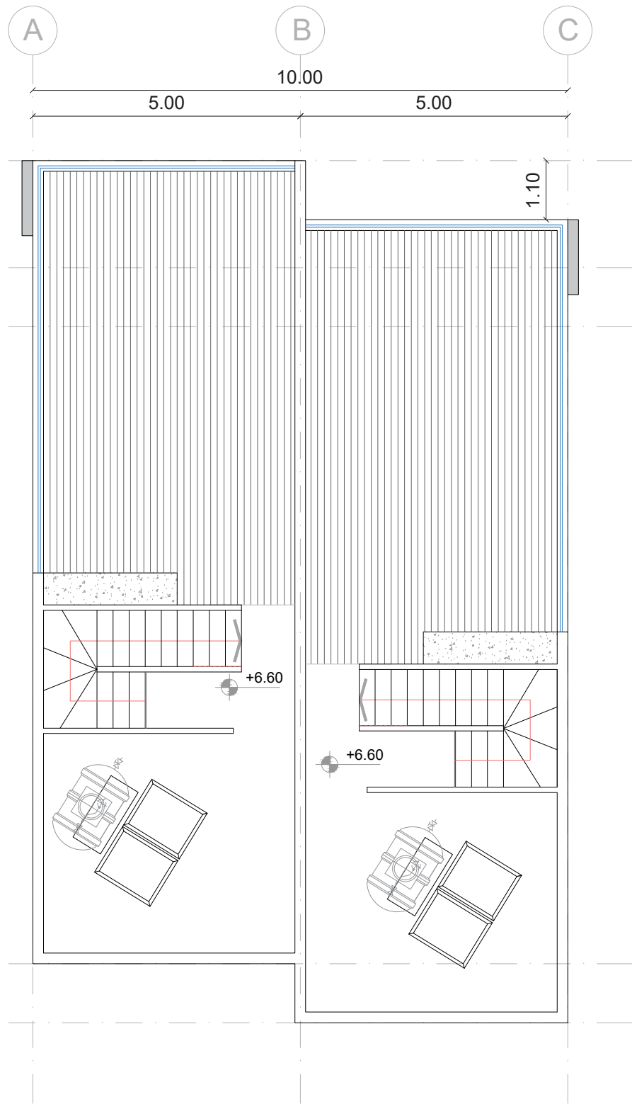
ROOF GARDEN
