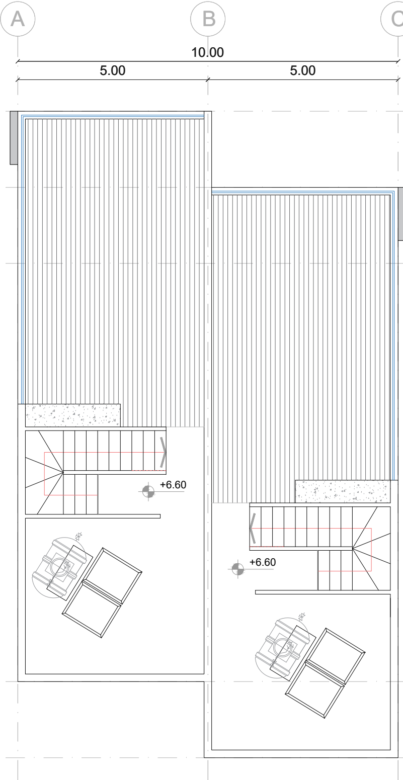
ROOF GARDEN
