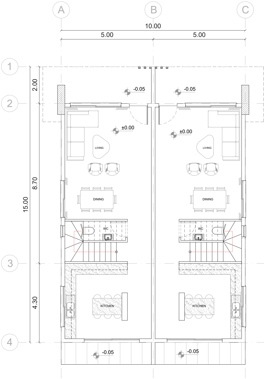
GROUND FLOOR
