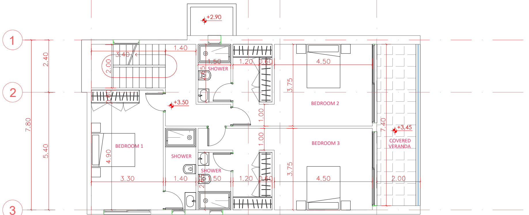
FIRST FLOOR - SCALE:1:100 HOUSE 1
