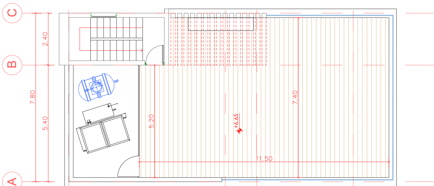
ROOF GARDEN - SCALE:1:100 HOUSE 1
