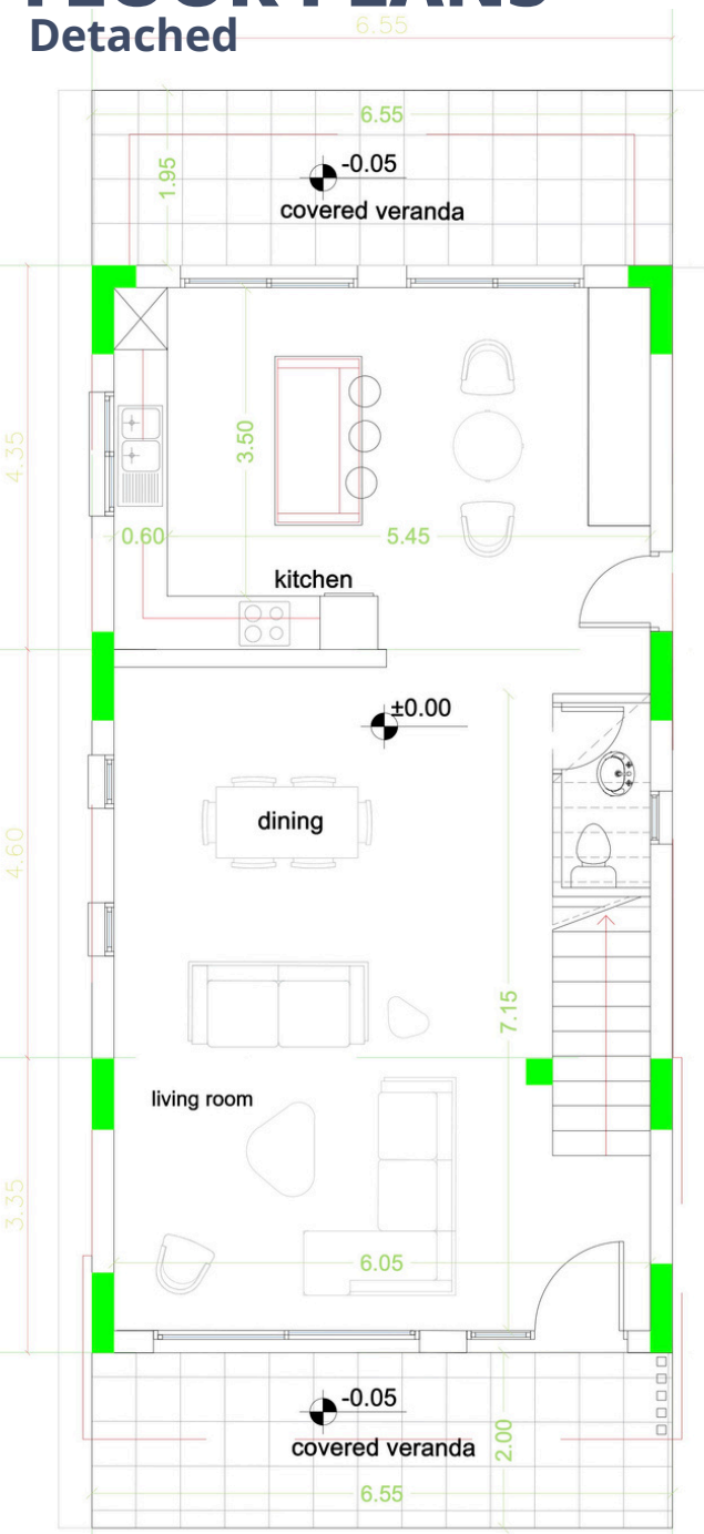
GROUND FLOOR
